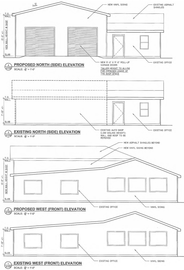
Above: Existing and proposed elevations
